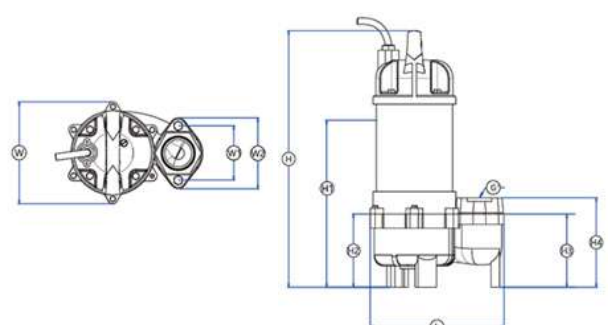
BIA-B75VA 700323
