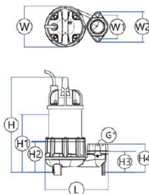
BIA-B40VA 700320
